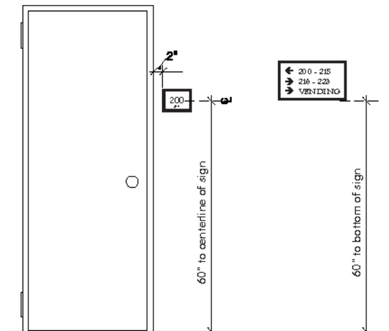
CORRIDOR SIDE ELEVATION (NOT TO SCALE)
